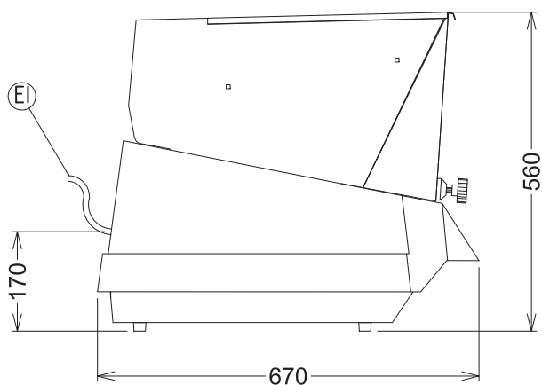
Lateral
